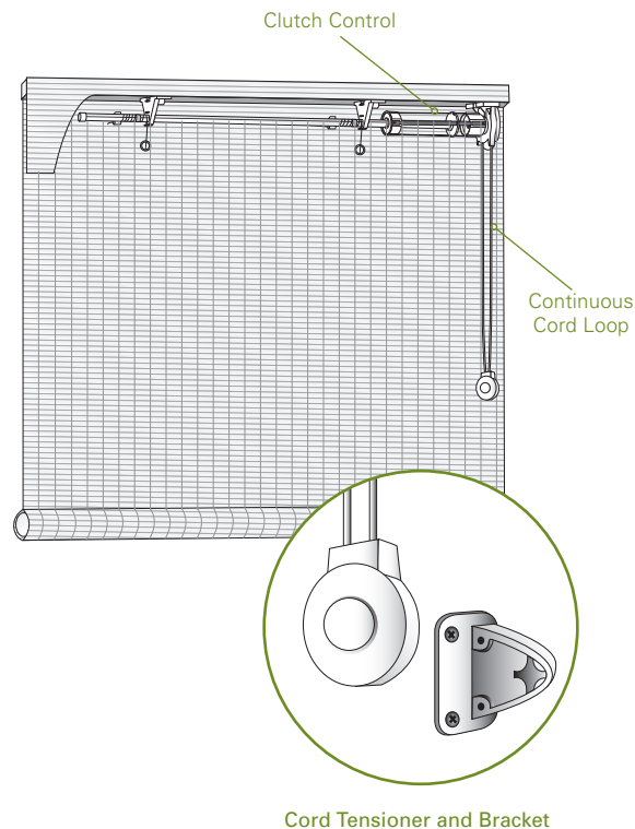
Cord Tensioner and Bracket
