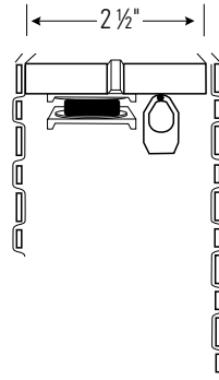
CORDLESS HEAD RAIL • Standard Shades • Waterfall Shades
