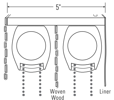
TWIN SHADE WITH 2 CLUTCHES Controls Same Side (shown) or Opposite Sides
