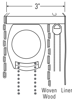
TWIN SHADE WITH CLUTCH (Clutch Control for Front Shade Only) Controls Same Side (shown) or Opposite Sides
