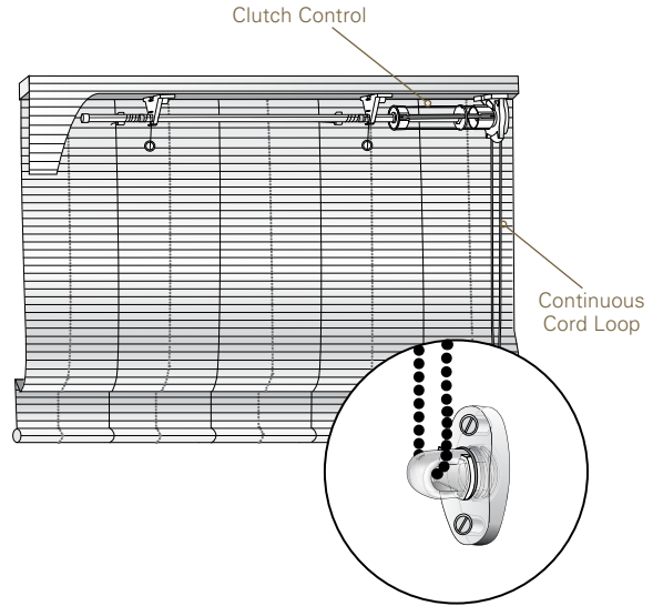
Cord Tensioner and Bracket
