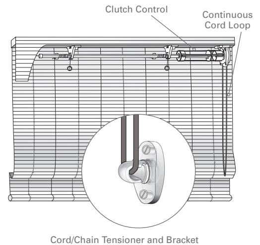
Cord/Chain Tensioner and Bracket
