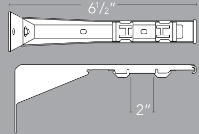
Double wall-mounted bracket
