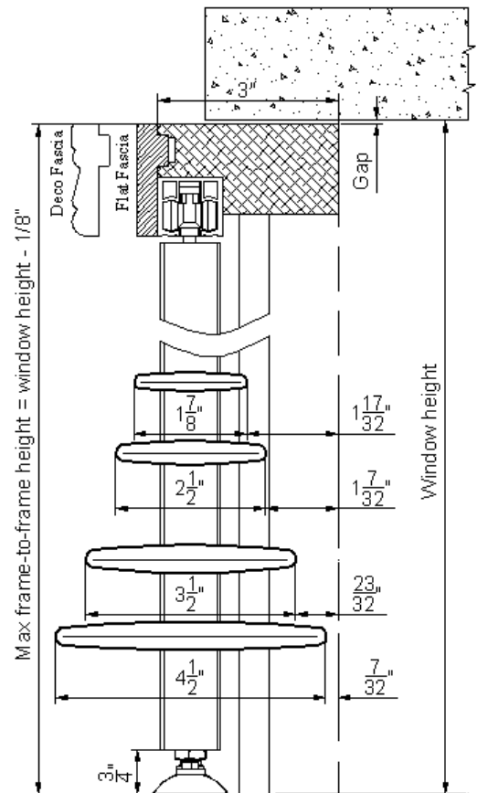
Semi-Inside Mount
