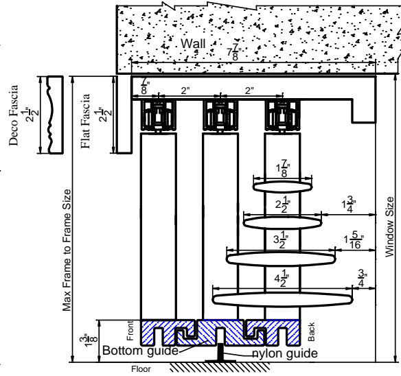
Inside Mount
